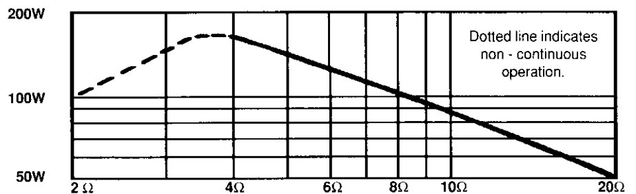
Graph of Max. Power Output Versus Load Impedance
